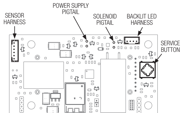
Bottle Filler Control Board Rear View
