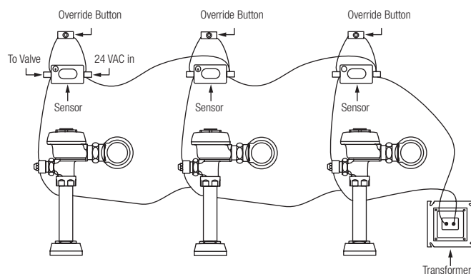
TYPICAL WIRING DIAGRAM FOR ONE OR MORE FLUSH VALVE(S)
