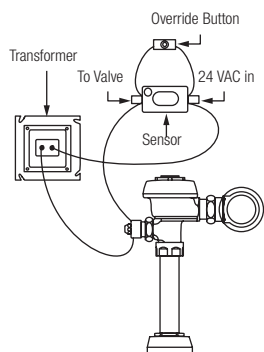
TYPICAL WIRING DIAGRAM FOR ONE FLUSH VALVE
